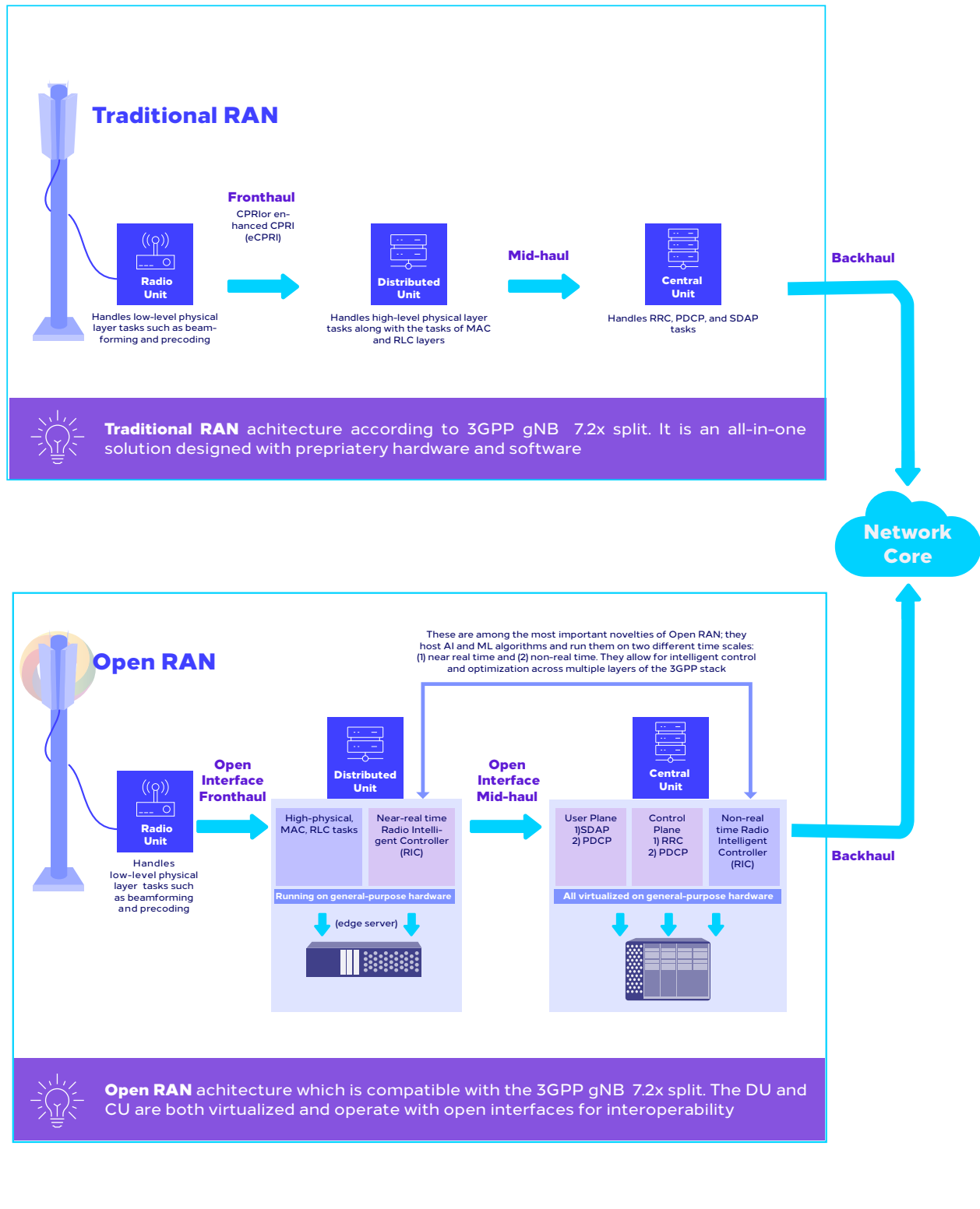
Figure 1: Illustration of Open RAN with a compare to traditional RAN. Both architectures are designed following the 3GPP gNB 7.2x split.
